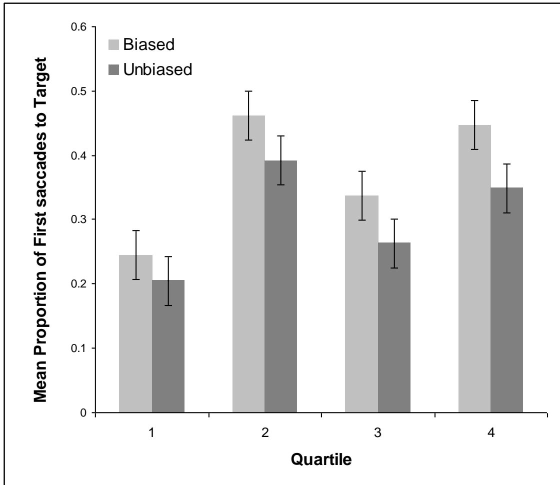
Figure 2. Proportion of first saccades to the target for the biased and unbiased sides across all 4 quartiles of Experiment 2. The display size in the first two quartiles was 6^\circ and in the third and fourth quartiles it was 10^\circ . Error bars represent 95% confidence intervals. Note that these are the conditional proportions calculated for the biased and unbiased sides separately.
