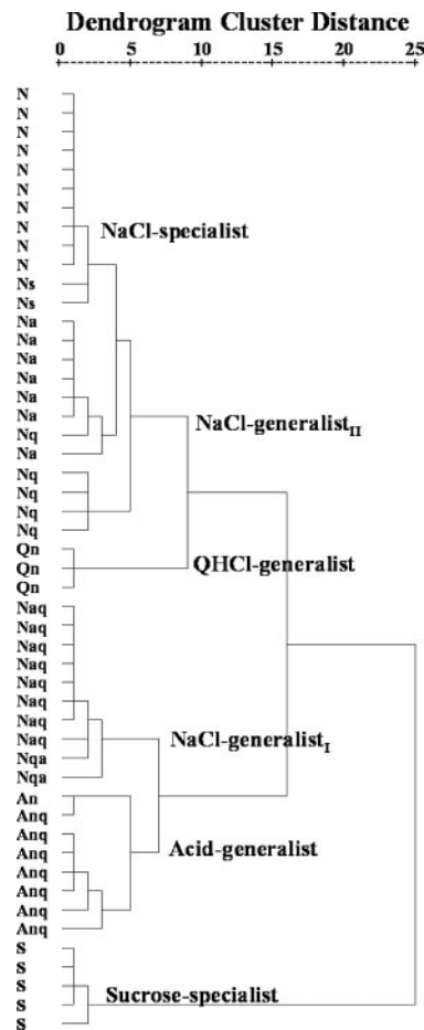
FIG. 2. Dendrogram showing the results of the hierarchical cluster analysis. Next to each neuron is the symbol of the taste stimulus (S, 0.05 M sucrose; N, 0.1 M NaCl; A, 0.01 M citric acid, and Q, 0.02 M QHCl) that evoked the best response, followed by the symbol(s) of other taste stimuli that evoked a response \geq 30\% of the best response.
